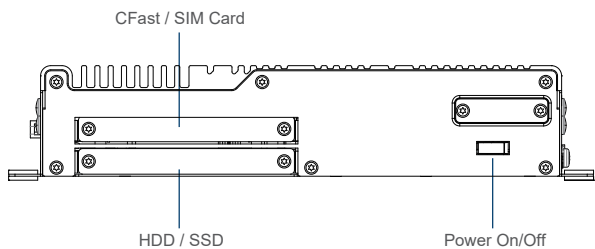
Rear I/O
