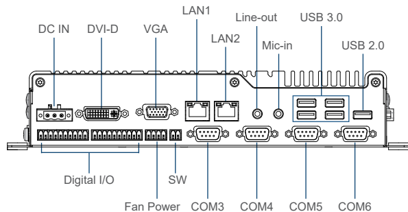
Front I/O
