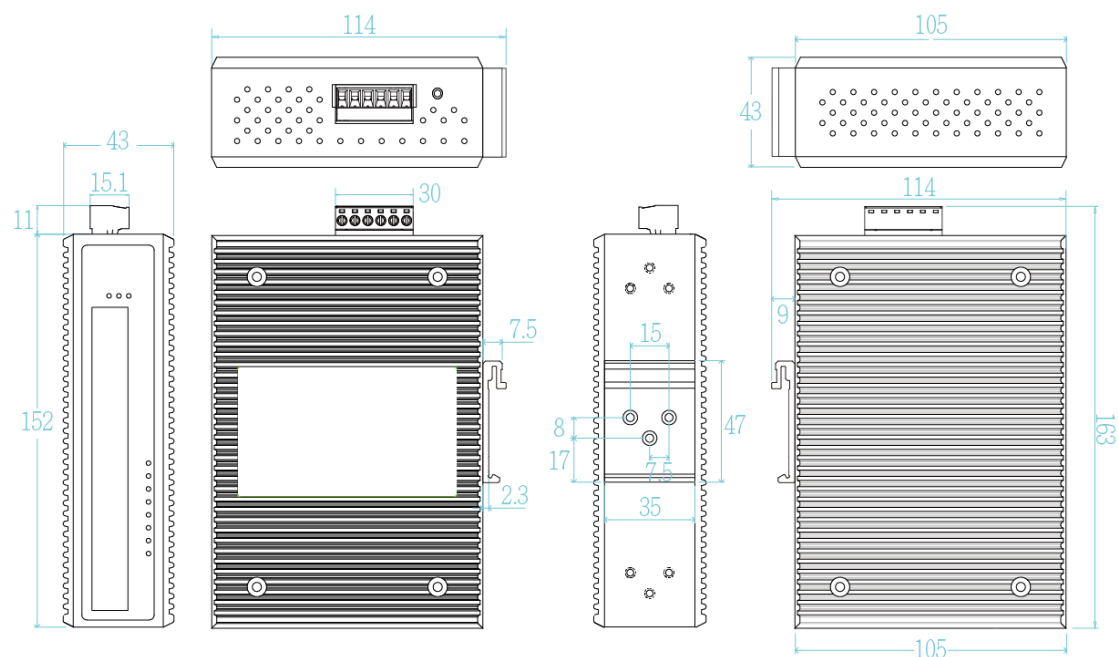
Non-PoE model
